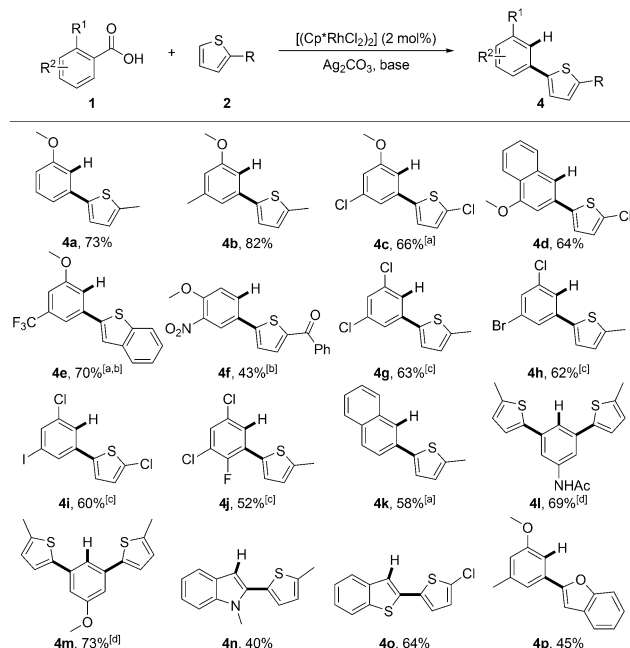
Scheme 4. Variation of the (hetero)aryl carboxylic acid. Reaction conditions: 1 (0.2 mmol), 2 (2 equiv), [(\text{Cp}^*\text{RhCl}_2)_2] (2 mol %), TEMPO (20 mol %), \text{Ag}_2\text{CO}_3 (3 equiv), \text{K}_2\text{HPO}_4 (1.5 equiv), NMP (2 mL), 100 °C, 24 h, then stirring for a further 6 hours at 140 °C. Yields of isolated products are given. [a] Stirring for a further 6 hours at 160 °C. [b] [(\text{Cp}^*\text{RhCl}_2)_2] (2 mol %), \text{Li}_2\text{CO}_3 (1.5 equiv), DMF. [c] [(\text{Cp}^*\text{RhCl}_2)_2] (4 mol %), \text{Li}_2\text{CO}_3 (1.0 equiv), DMF. [d] 2 (4 equiv), [(\text{Cp}^*\text{RhCl}_2)_2] (2 mol %), \text{Ag}_2\text{CO}_3 (6 equiv), DMF.
